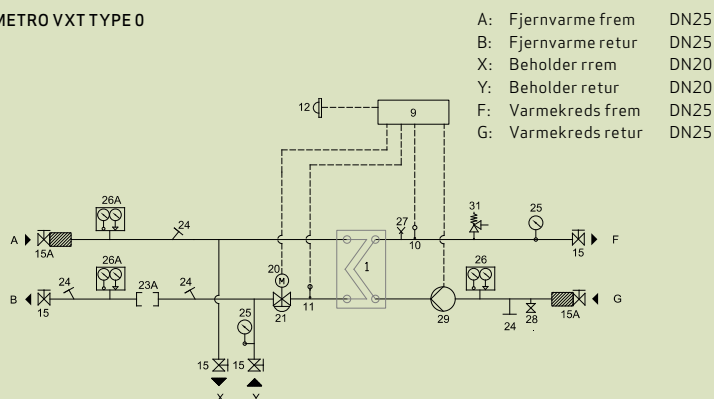
METRO VXT TYPE 0
