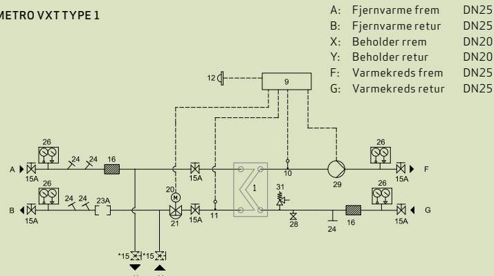
METRO VXT TYPE 1
